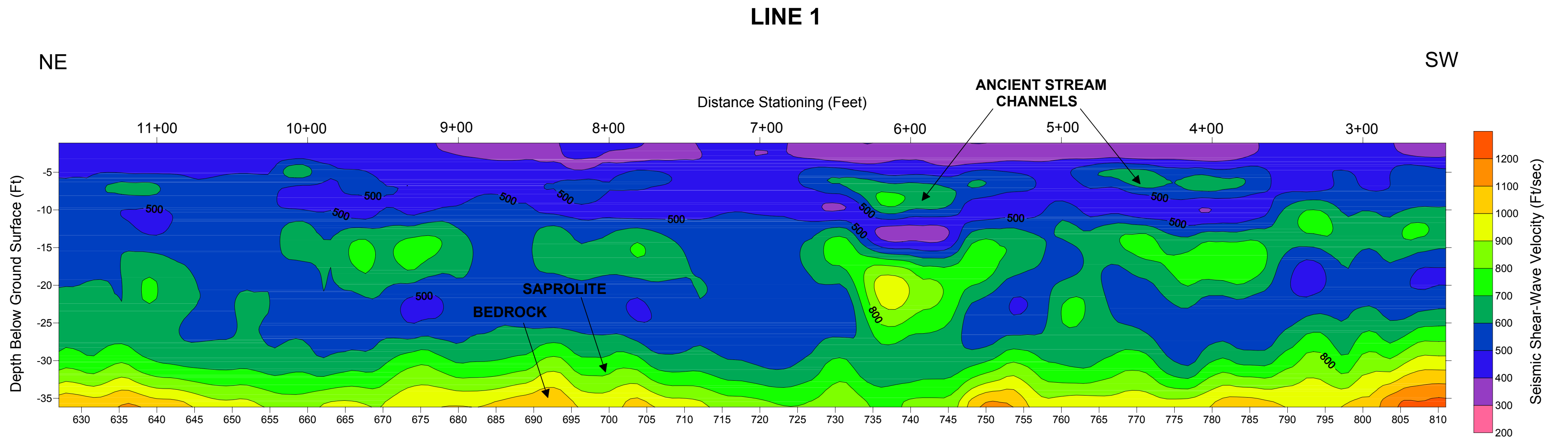
Estimated Shear-Wave Velocity Profile Based on SurfSeis Modeling of MASW Survey Data Horizontal Scale 1 inch= 50 Ft Vertical Exaggeration x 5
