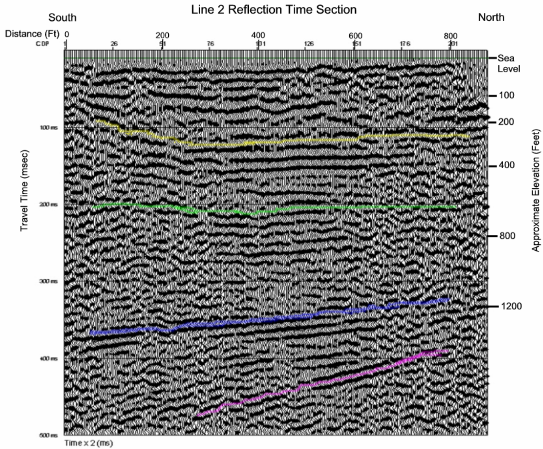
Seismic reflection profile recorded in a noisy urban area near the Santa Barbara Airport. This 850-foot long profile was recorded in one-day using an accelerated weight-drop seismic energy source. The yellow and green reflection patterns show layering within the Quaternary Santa Barbara formation. The blue and purple patterns show Monterey Formation layering.
